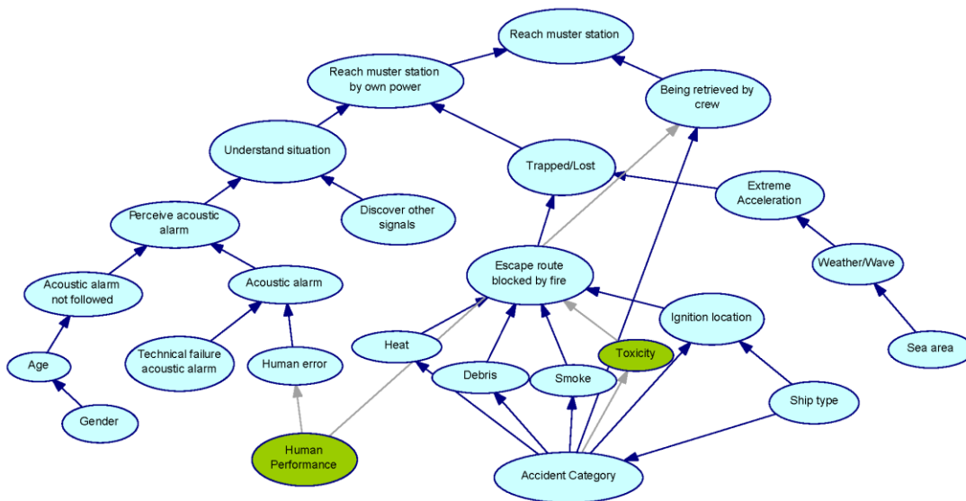
Figure 3. Bayesian network for Reaching Muster Station (fire/explosion)
